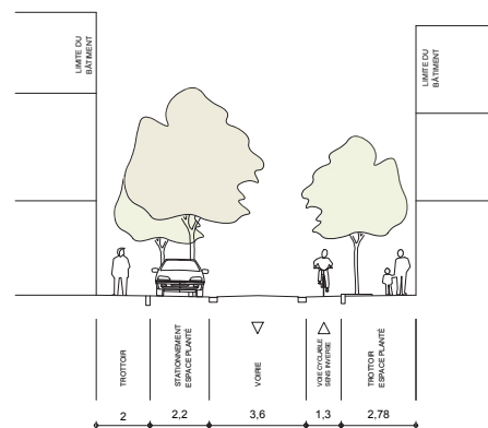
Rue Brichaut : suggestions Brichautstraat: suggesties
